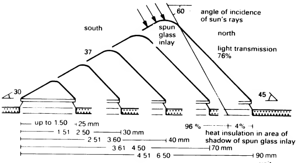
⑬ Saw-tooth glass fibre-reinforced polyester skylight
